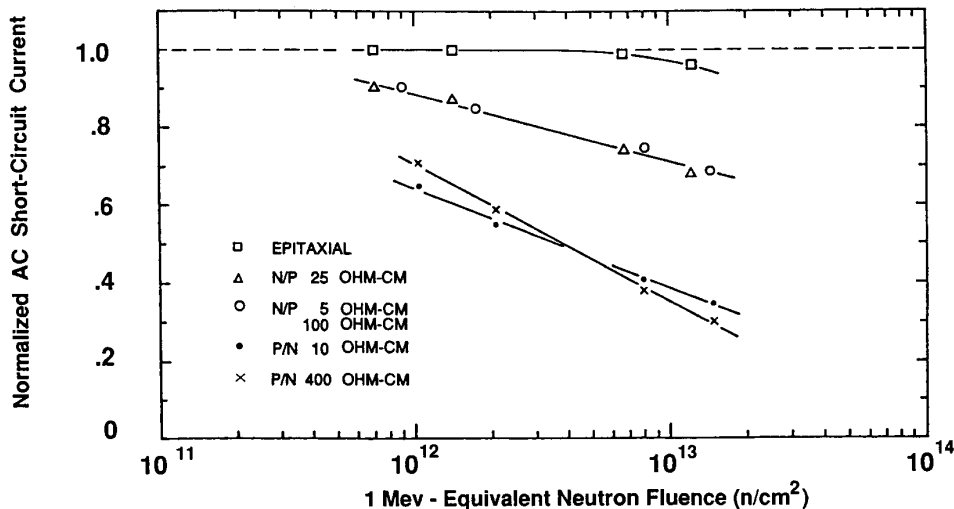
Figure 2. Photodiode AC Short-Circuit Current Versus Neutron Fluence
