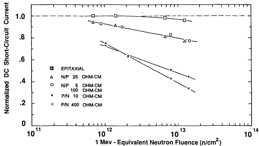
Figure 1. Photodiode DC Short-Circuit Current Versus Neutron Fluence
