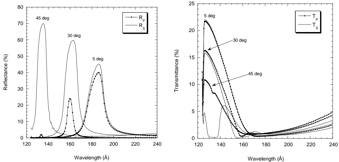
FIGURE 4. The reflectance and transmittance of the multilayer coating on the photodiode.
