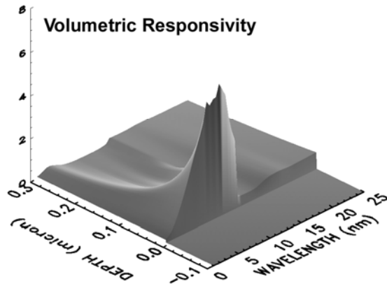
Figure 2. The calculated volumetric responsivity (in units of A/W\mu m ) of the photodiode as a function of the incident wavelength and the depth into the device.
